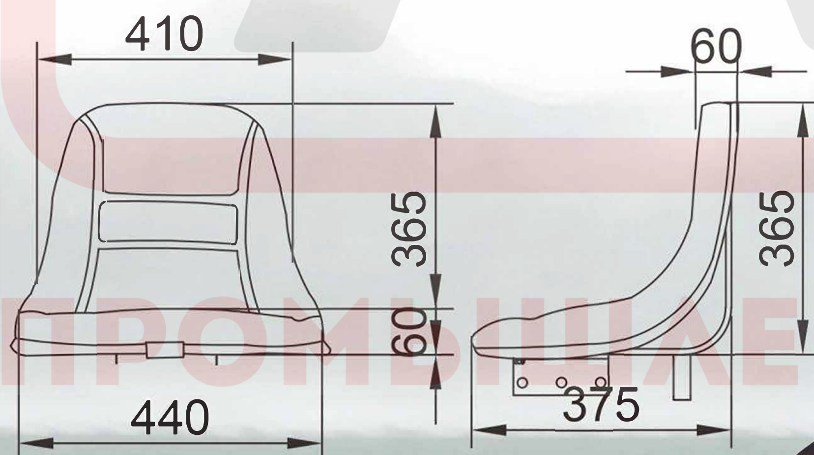
型号:FD-826 MODEL:FD-826
