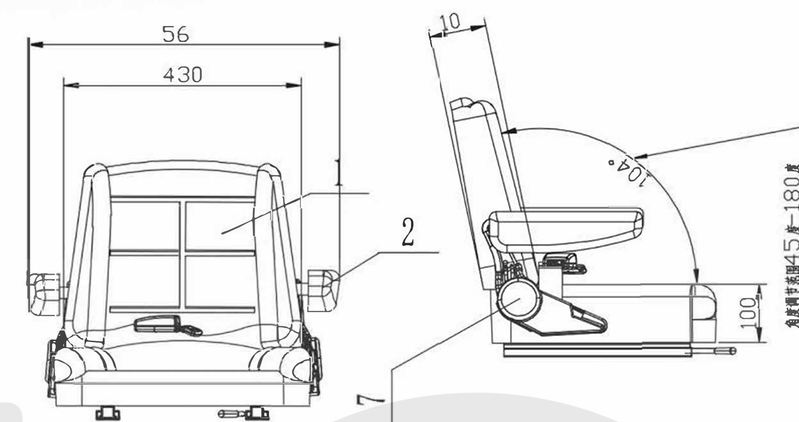
型号:FD-820 MODEL:FD-820
