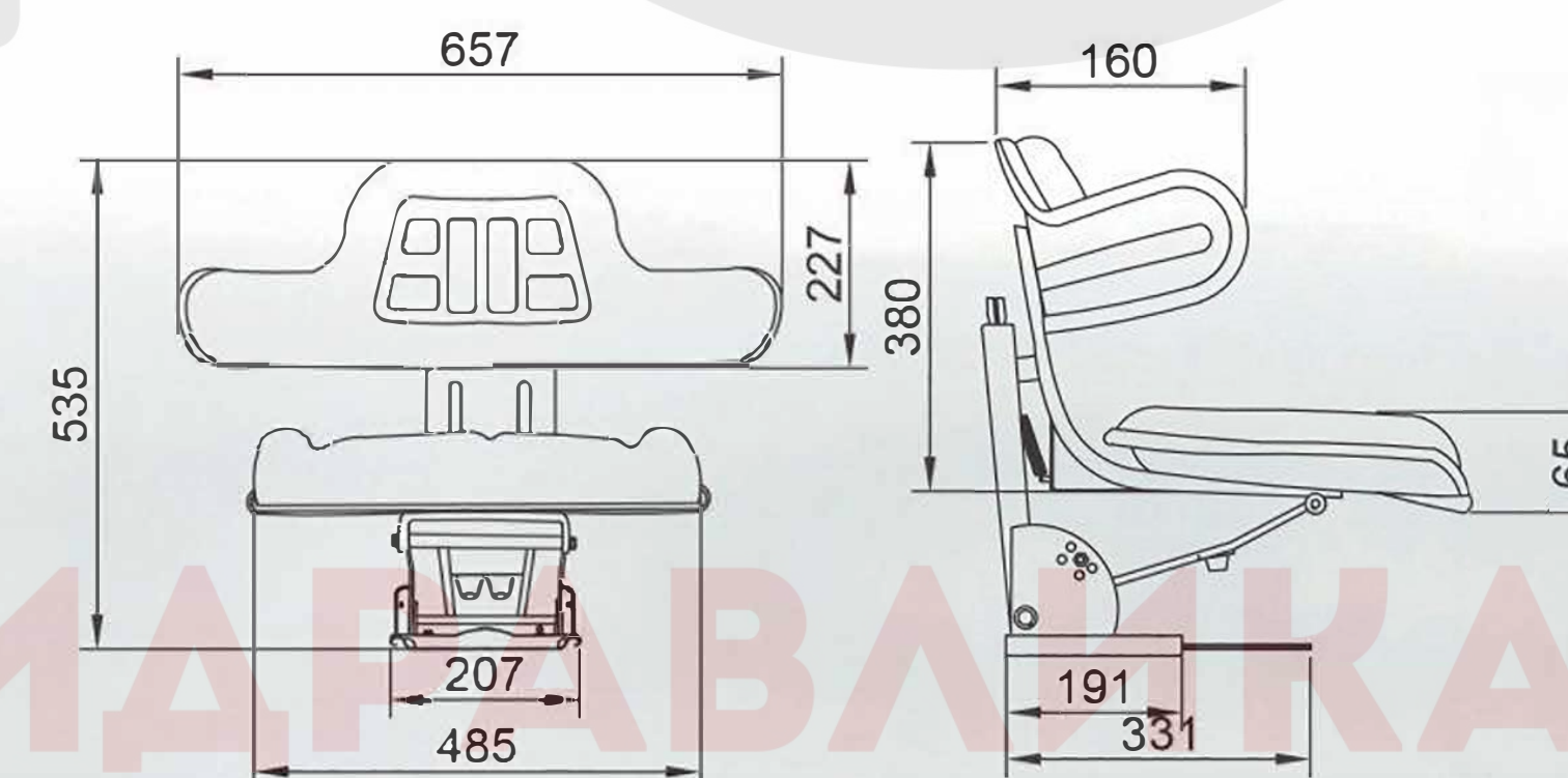
型号:FD-810 MODEL:FD-810
