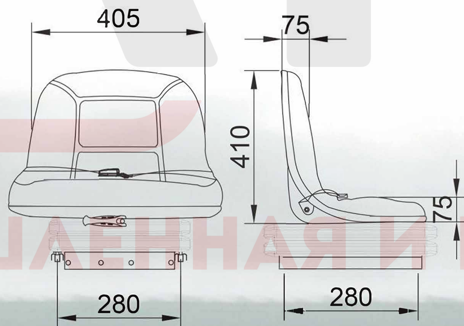
型号:FD-858 MODEL:FD-858
