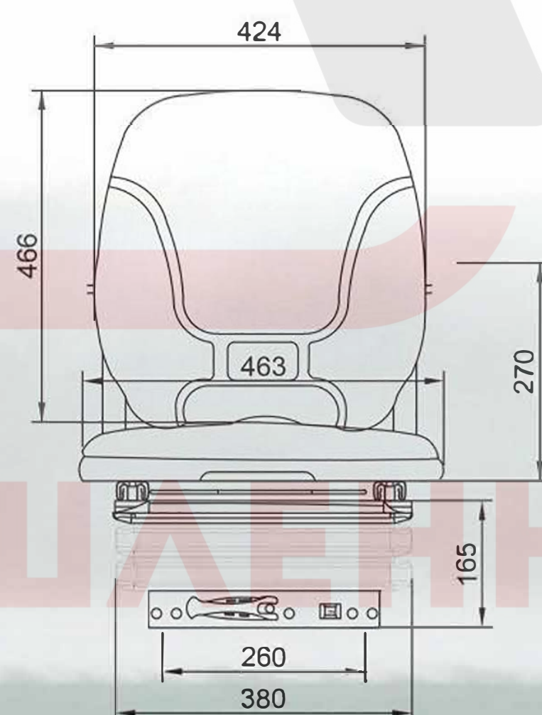
型号:FD-856 MODEL:FD-856
