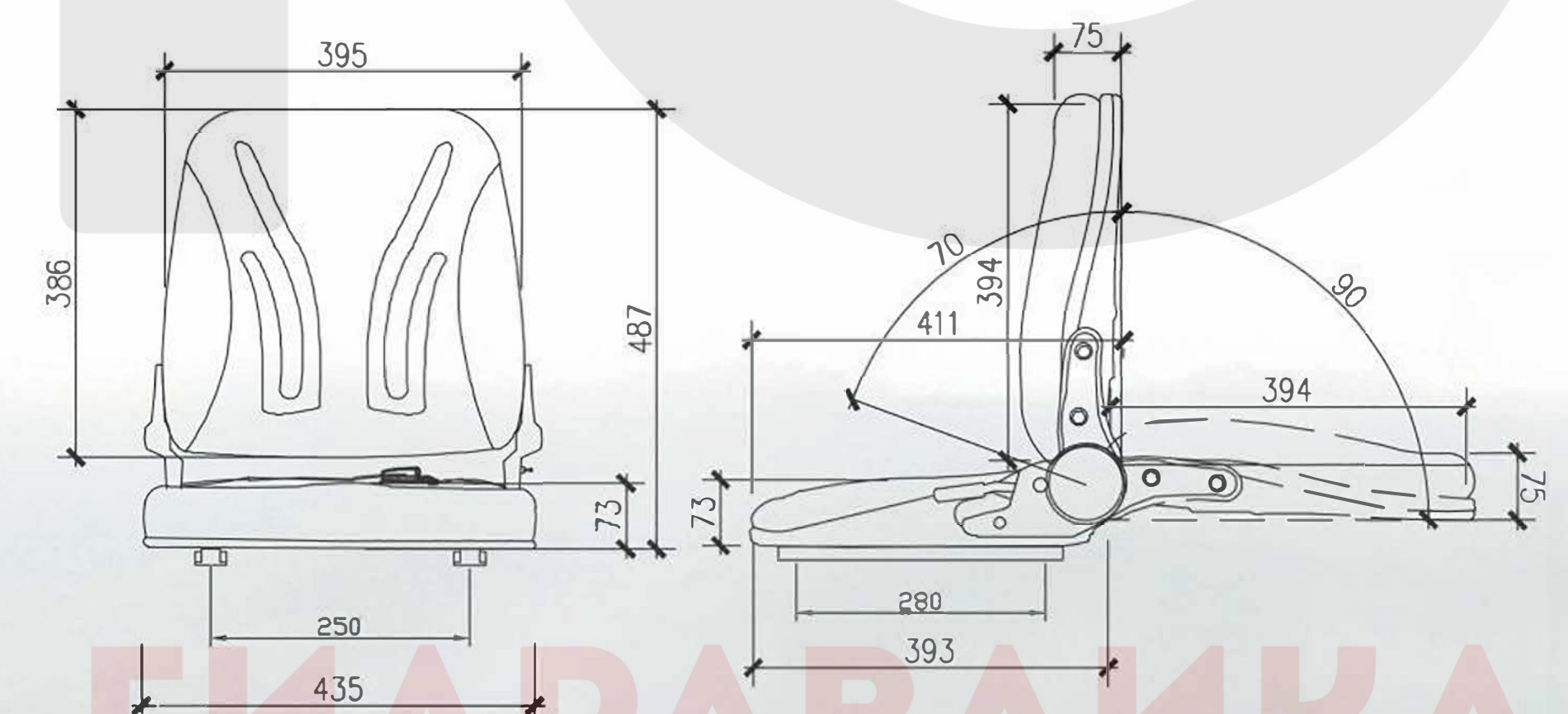
型号:FD-832 MODEL:FD-832
