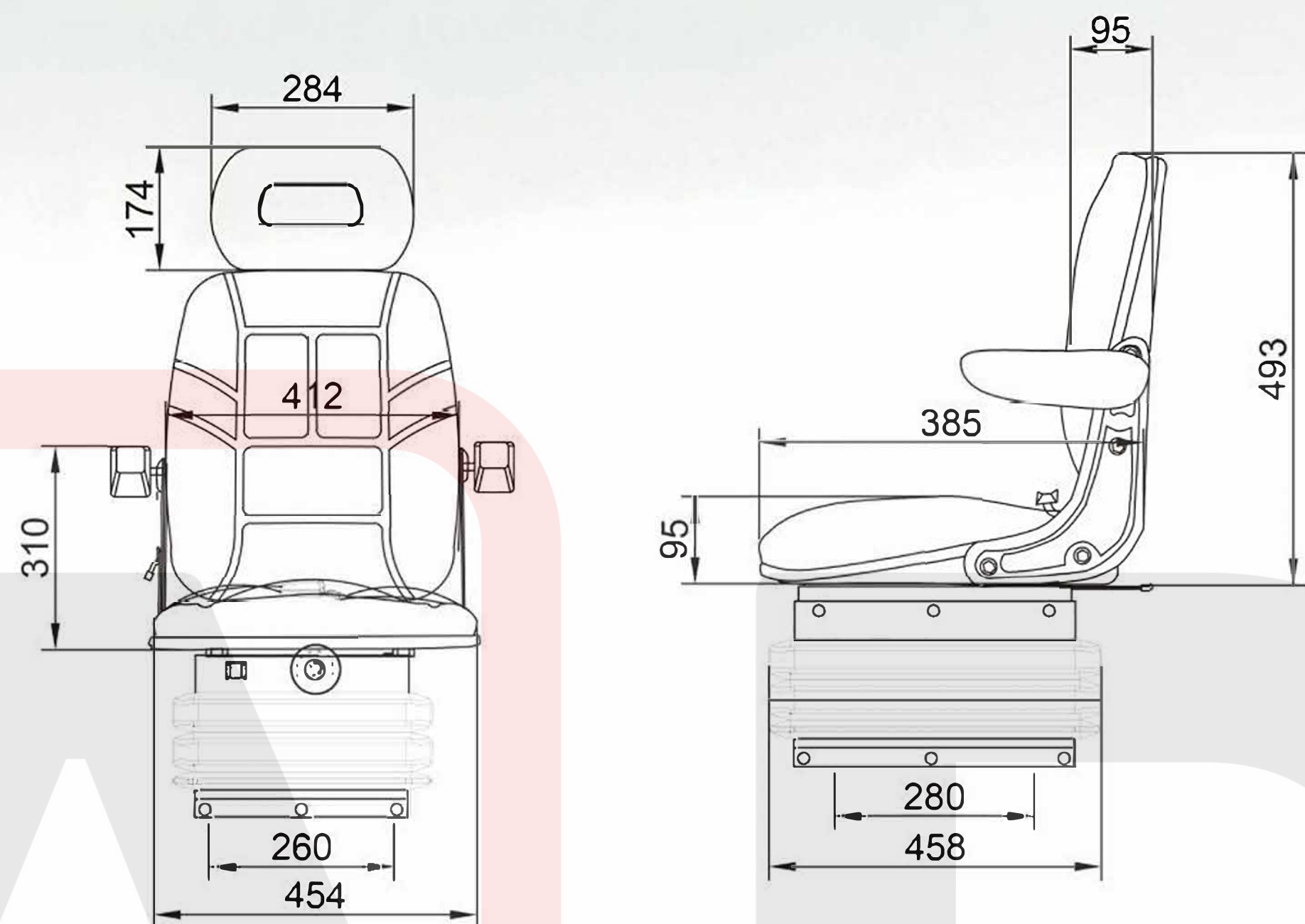
型号:FD-853 MODEL:FD-853
