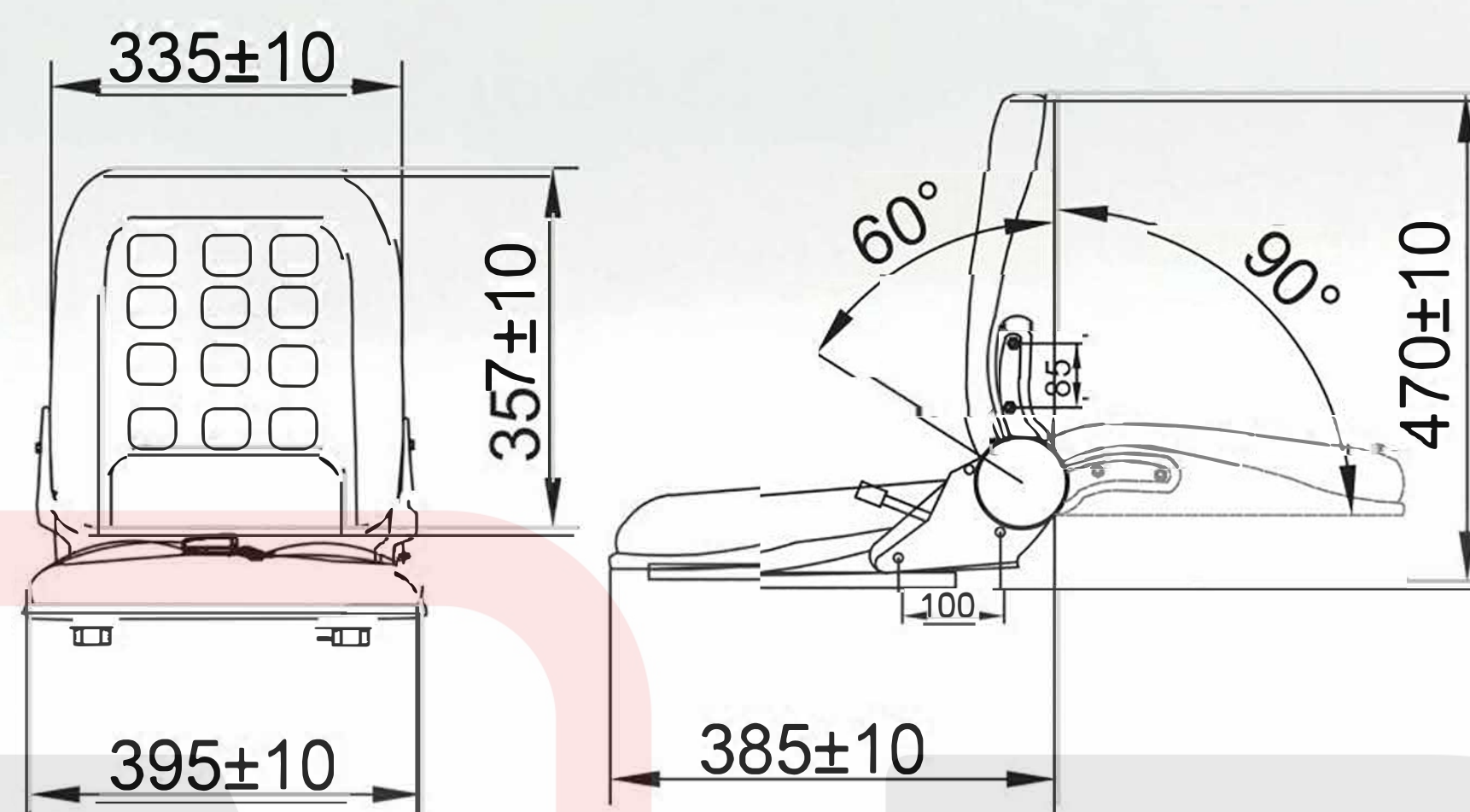
型号:FD-816 MODEL:FD-816
