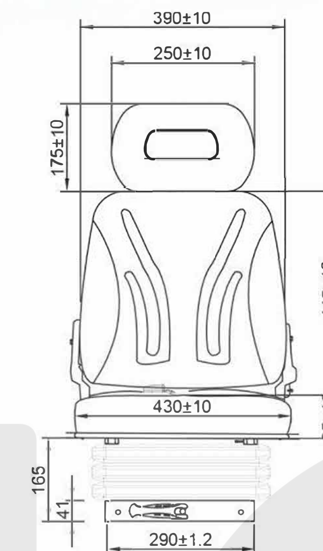
型号:FD-802 MODEL:FD-802
