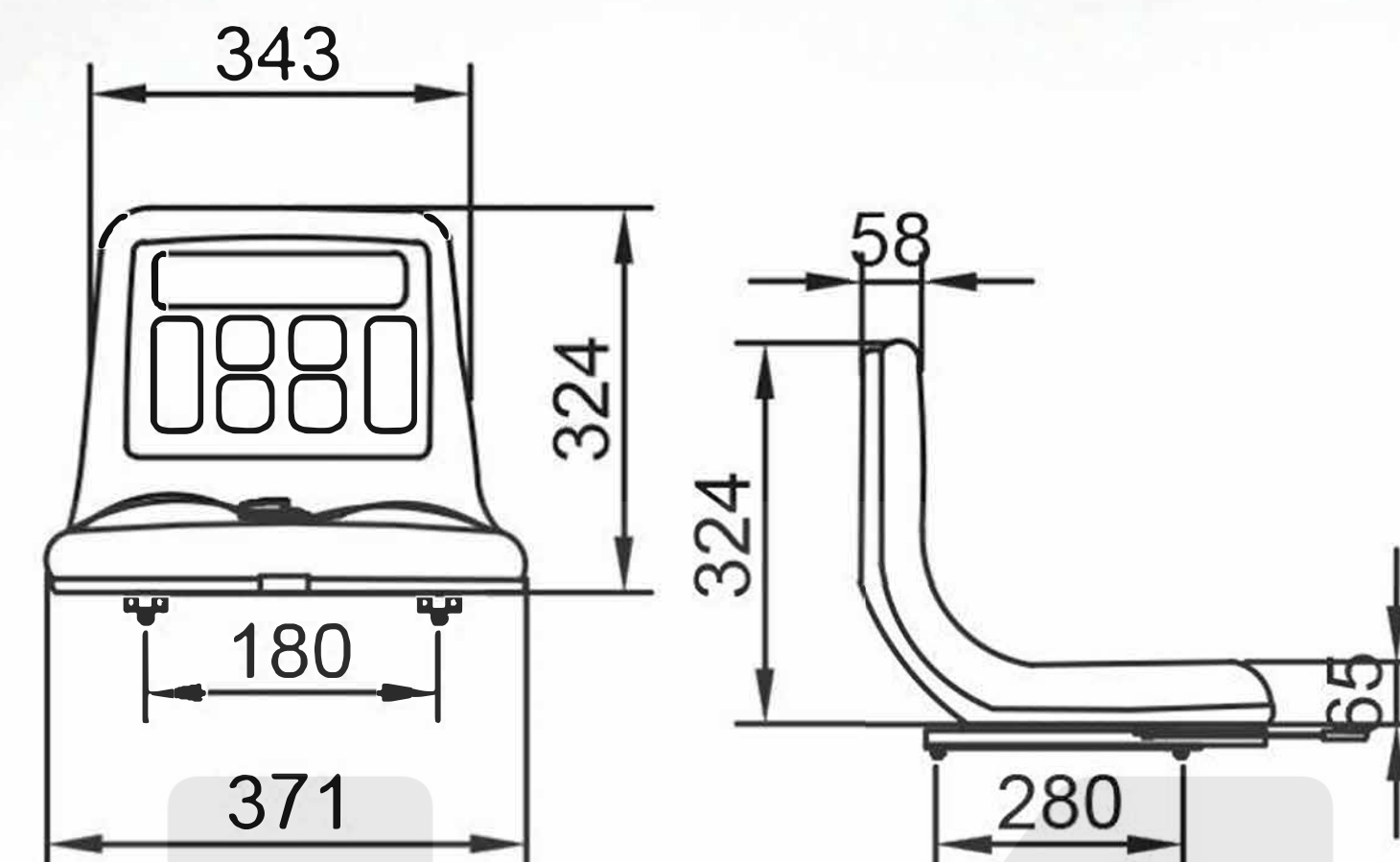
型号:FD-811 MODEL:FD-811
