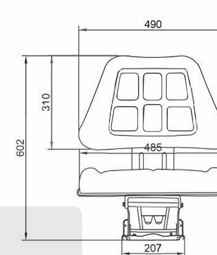
型号:FD-810 MODEL:FD-810
